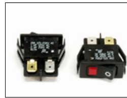
1290030 SW-Rocker-DPST-16A-Lit-Red-250V
