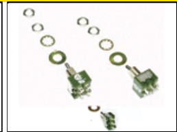
1290016 SW-Toggle-Miniature-DPDT-6A
