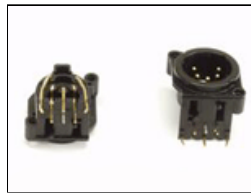
1270158 CT-Xlr-PCB-Male-5-Pin-Right-Angle
