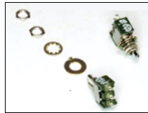
1290013 SW-Toggle-Miniature-SPDT-5A
